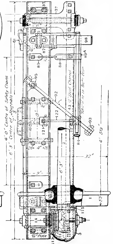
Fig. 4646. Half Cross Section and Half End Elevation.
